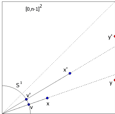
Fig. 6. Construction to determine the symmetrized spread in Lemma 6: the points x and x' in \mathcal{Y}_n^{(2)} are contained in the cube [0, n - 1]^2 and their normalizations v, v' in \mathbb{S}^1 .
